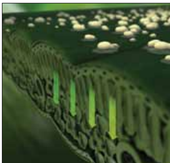
Translaminar Movement
