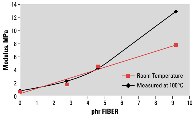
Modulus at 25% Elongation Machine Direction
