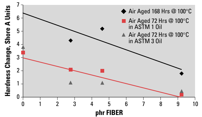
Hardness Change
