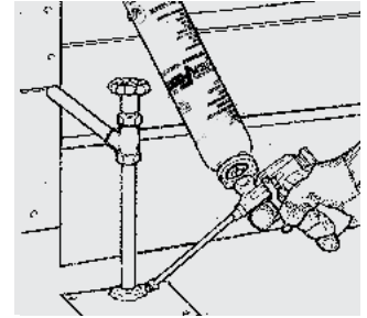
Fireplace gas line
