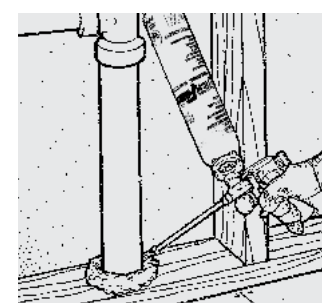
Sewer plumbing penetration
