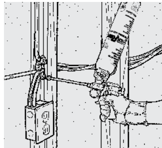
Electrical wire penetration
