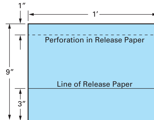
9" FlexWrap™ (for greater than 4" recesses, double stud framing)
