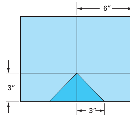
9" FlexWrap™ (for greater than 4" recess, double stud framing)
