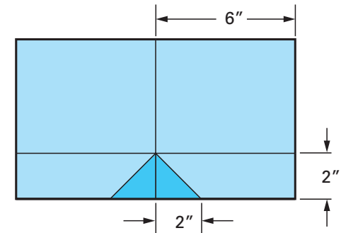
6" FlexWrap™ (for greater than 4" recesses, single stud framing)
