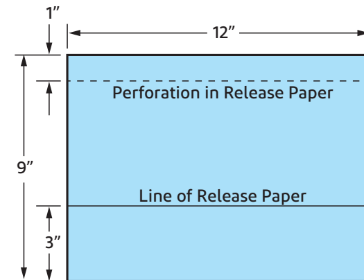
9" FlexWrap™ (for greater than 2" recess, double stud framing)
