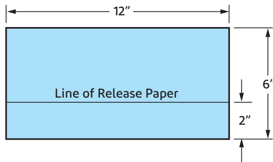
6" FlexWrap™ (for up to 2" recess, single and double stud framing)
