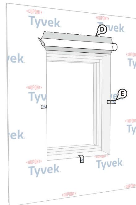
Alternate Method to Secure Head Flap
